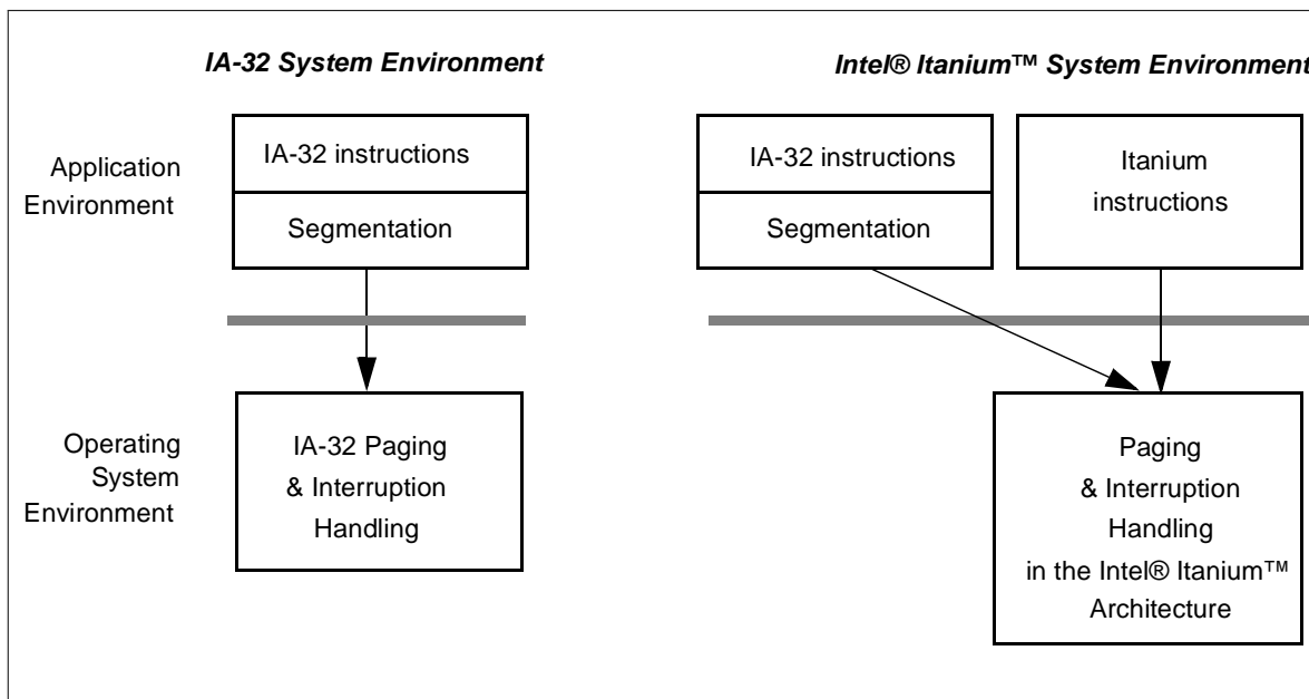
Figure 2-1. System Environments
