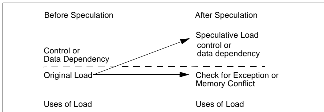
Figure 3-2. Speculation Model in the Intel® Itanium™ Architecture
