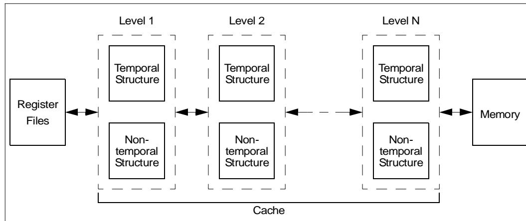
Figure 4-4. Memory Hierarchy
