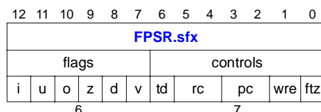
Figure 5-3. Floating-point Status Field Format
